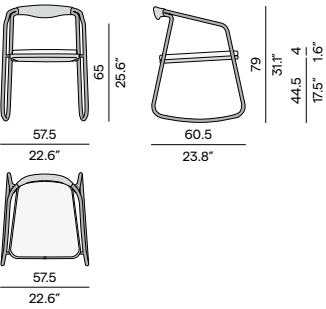
Rocking chair / RC02
