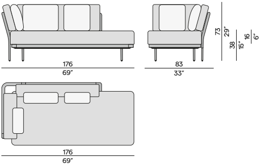
Right corner double end seat / CDRES001
