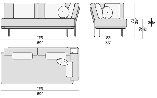
Left corner double seat / CDLS001
