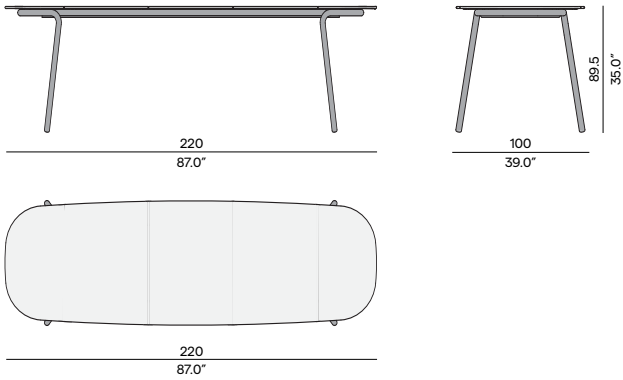
High dining table / 220×100
